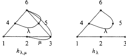
Figure 1. The diagrams of the forms h_{\lambda,\mu} and h_\lambda .
